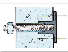
Réhabilitation plaque apparente
