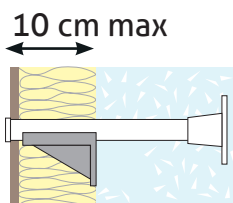
Réhabilitation plaque apparente
